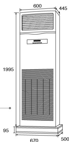
BFG-100PV BFG-125PV BFG-150PV
